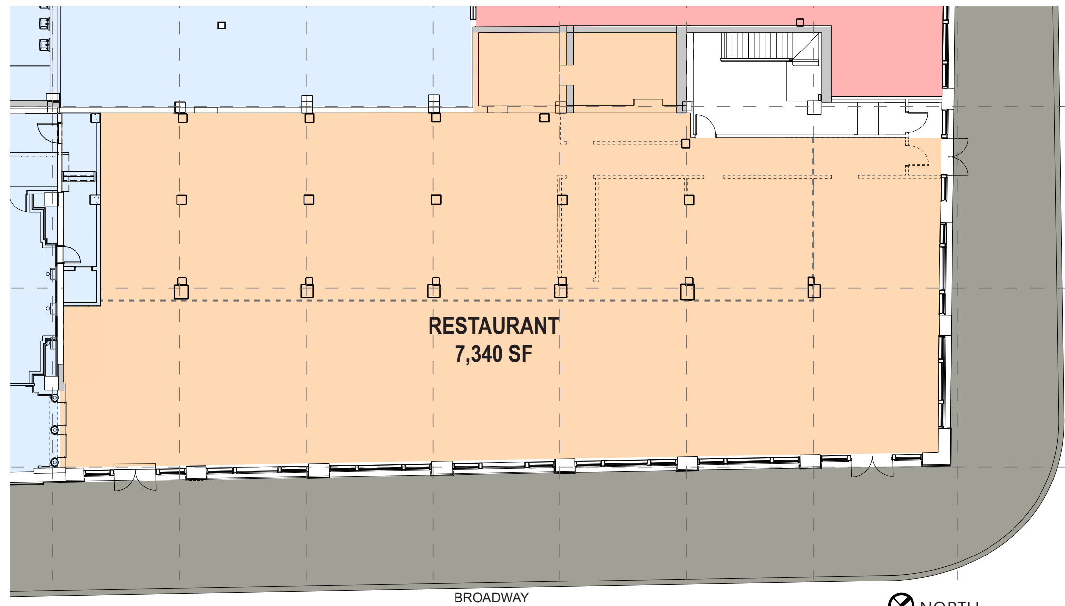
ENLARGED PLAN
